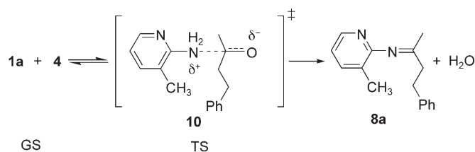
Scheme 2. Increase of the polarity of the system during the progress of the reaction from the ground state (GS) towards the transition state (TS).
