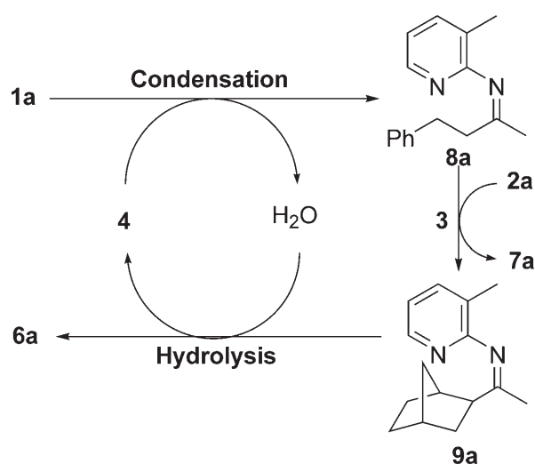
Scheme 1. Mechanism of chelation-assisted C–C bond activation of 1a with norbornylene ( 2a ).
