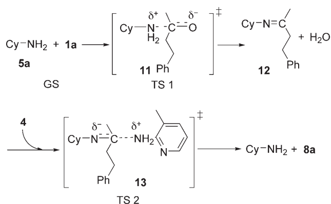
Scheme 3. Increase of the polarity system during the progress of the reaction from the ground state (GS) towards the transition state (TS).
